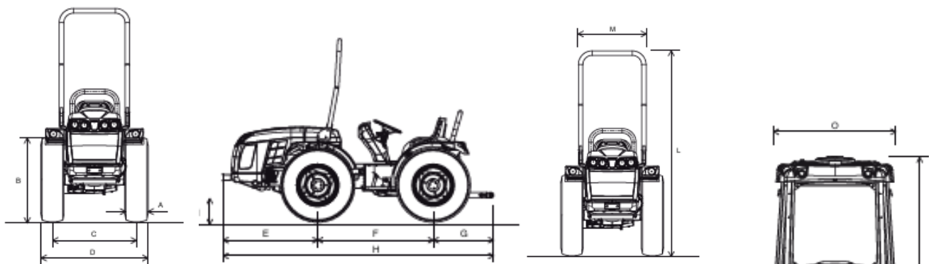
TRACTOR DIMENSIONS INVICTUS K600 AR (mm):
